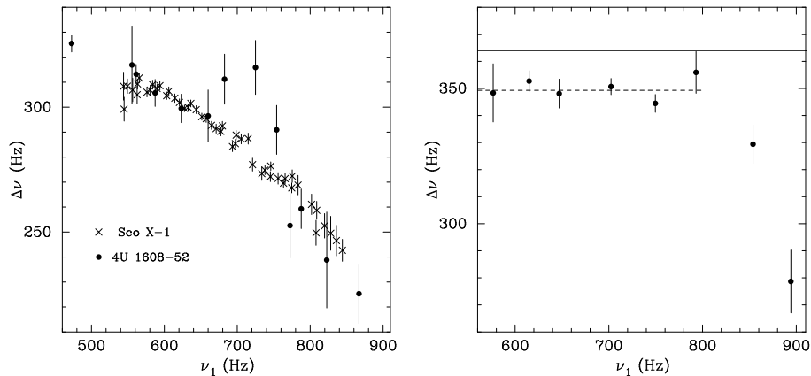
Figure 3. Left Panel: Frequency separation between the two simultaneous kHz QPOs in 4U 1608-52 (circles) and Sco X-1 (crosses). Right Panel: Frequency separation between the two simultaneous kHz QPOs in 4U 1728-34 (circles). The solid line indicates the frequency of the burst oscillations at 363.95 Hz (Strohmayer et al. 1996). The dashed line indicates the average value of \Delta\nu (349.3 Hz) for the first 6 points. For the three sources \Delta\nu as a function of \nu_1 was calculated as explained in the text.
